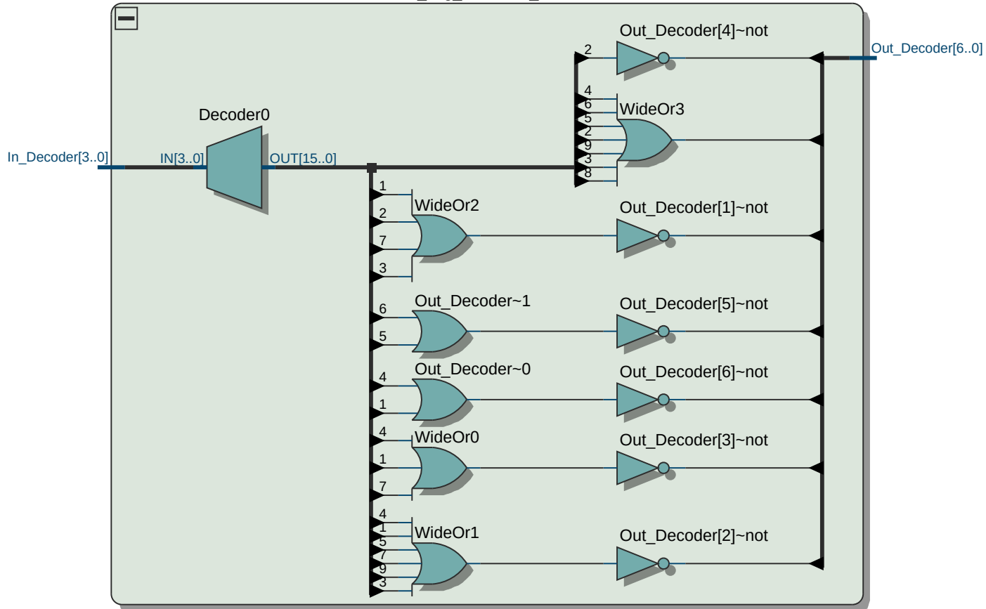
seven_seg_D:Pcount_Decoder
